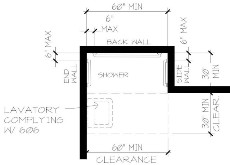
FIGURE 611.7(A) ROLL-IN SHOWERS FOR ASSISTED BATHING OPTION 1
