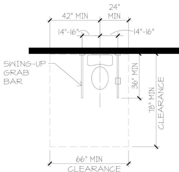
FIGURE 611.5 ASSISTED USE WATER CLOSET
