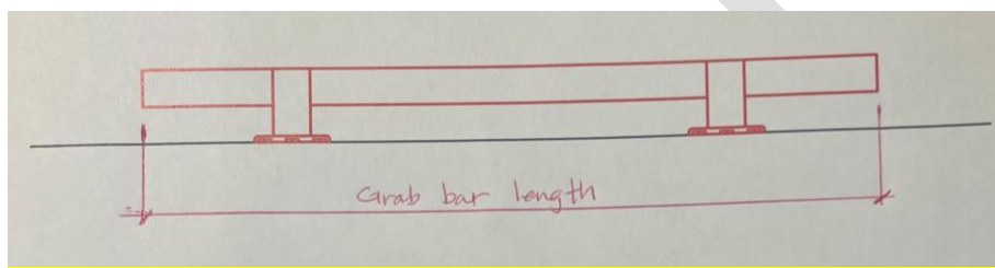
Figure 609.7.2(B) GRAB BAR LENGTH - EXAMPLE OR EXCEPTION
