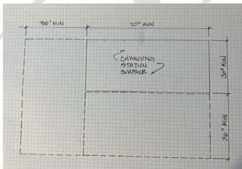
Figure 615.7 SIZE AND MANEUVERING CLEARANCES AT THE CHANGING SURFACE OF THE ASSISTIVE TABLE
