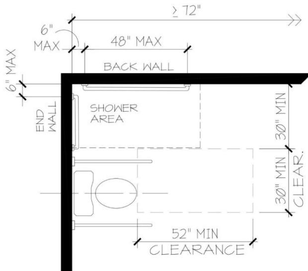
FIGURE 611.7(C) ROLL-IN SHOWERS FOR ASSISTED BATHING OPTION 3
