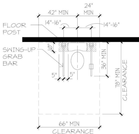
FIGURE 611.5.6 ASSISTED USE WATER CLOSET FLOOR-MOUNTED SUPPORT POSTS
